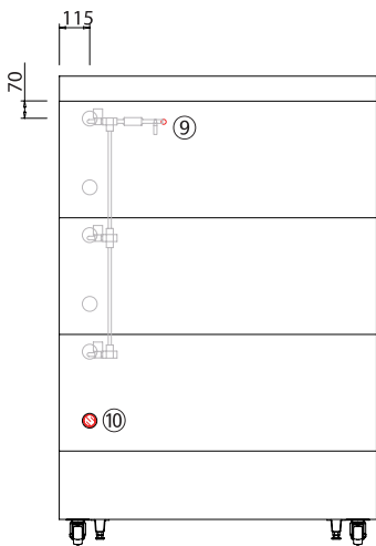
배면 / REAR VIEW
