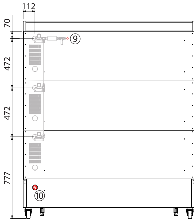
배면 / REAR VIEW
